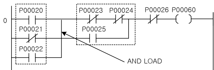
[Ladder Program]
