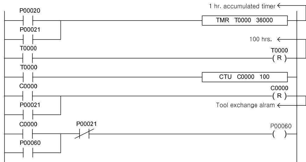
[Ladder Program]
